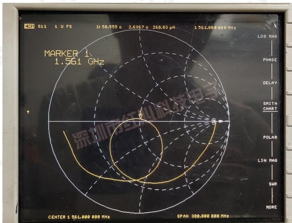
Smith Chart (史密斯圆图)
